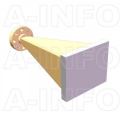
LB-10-25-ASPO Standard Gain Horn Antenna 75-110GHz 25dB Gain Rectangular Waveguide Interface
